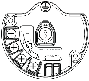
648 Wireless Sensor Connections Diagram
